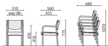
MC-510BR
