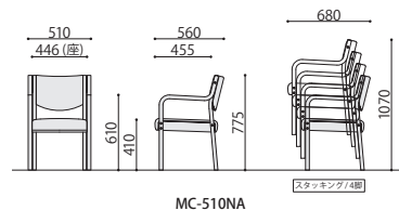
MC-510NA
